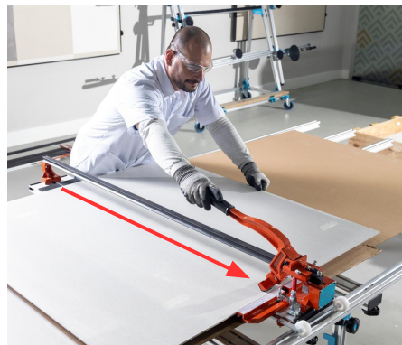
Image 55: Complete the score by pushing the diamond blade from one end to the other.
