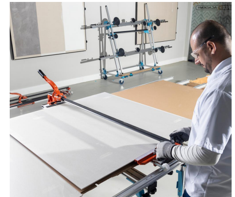
Image 51: Fit the piece in the scorer so that it is stable.
