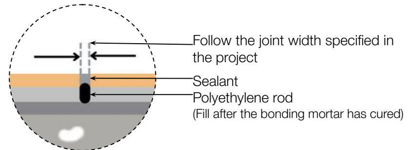
Detail 02
