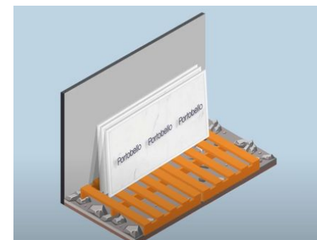
Image 07: After offloading the pallets, store the parts on a level surface, in a vertical position.
