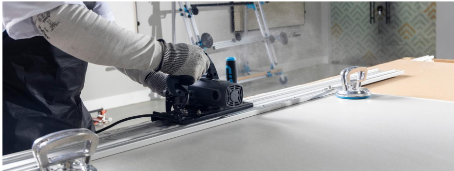
Image 77: Slide the marble saw along the rail, without forcing the disc to advance across the piece.
