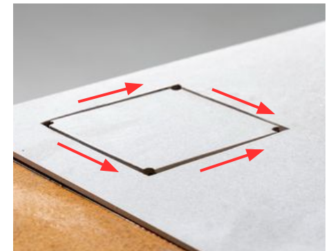
Image 83: The cut should be made in the direction of the largest area of the piece.
