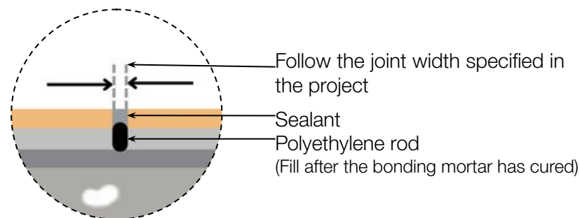
Detail 02
