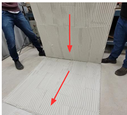
Image 29: Open mortar grooves in the same direction.
